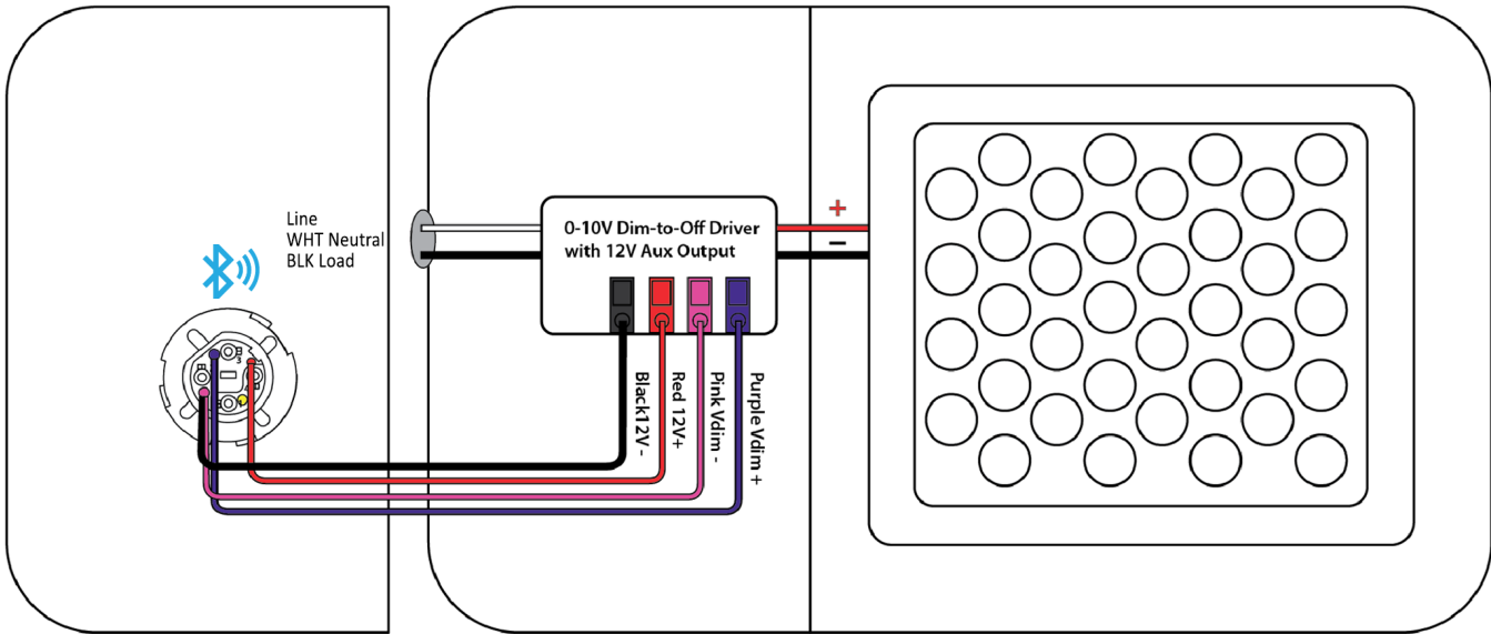
ZKV-R1L Receptacle on outside of fixture
